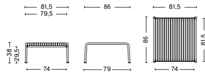
PALISSADE LOW TABLE Length 81,5 cm Width 86 cm Height 38 cm
