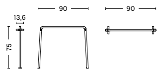
PALISSADE MIDDLE LEG Width 90 cm Depth 13,6 cm Height 75 cm
