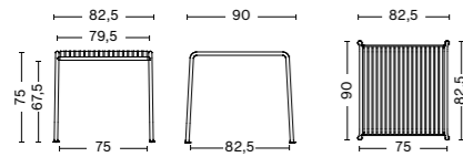
PALISSADE TABLE Length 82,5 cm Width 90 cm Height 75 cm
